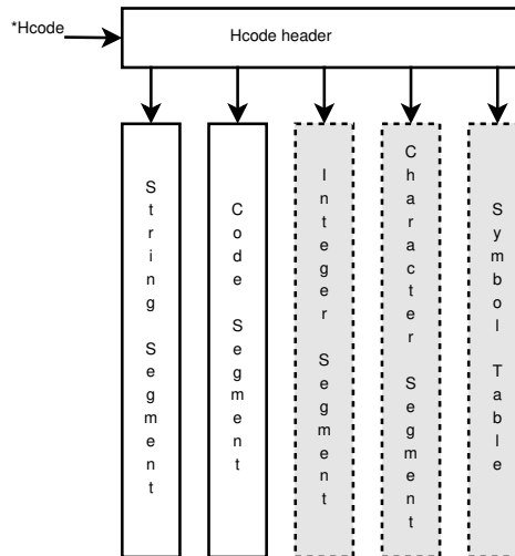
Figure 2.3: Hcode structure
