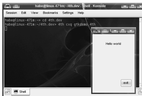
Figure 13.1: GTK demo
