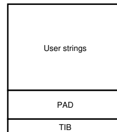
Figure 9.1: Character segment
